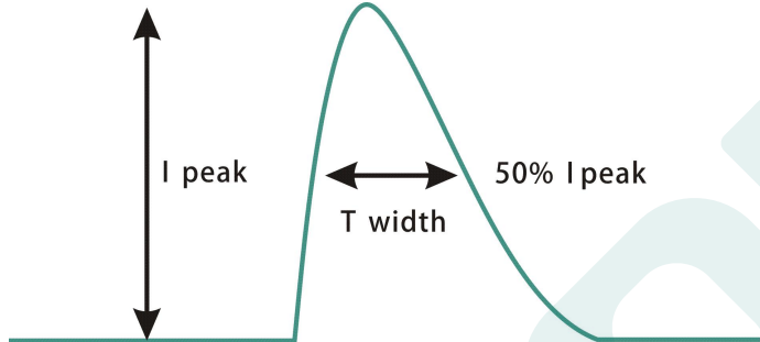
Inrush current(DL-150W-DX-MXG)
