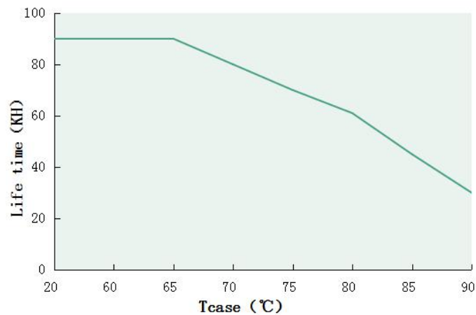
Tcase VS Lifetime(DL-150W-DX-MXG)
