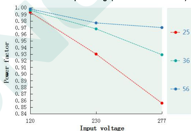
Power factor VS Input voltage(DL-150W-V56DX-MXG)
