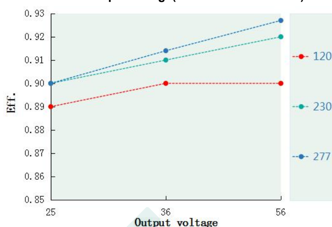
Eff. VS Output voltage(DL-150W-V56DX-MXG)
