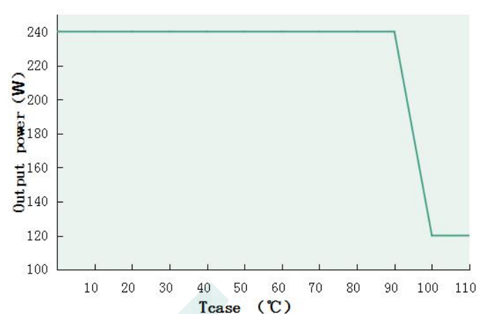
Output power VS Tcase (DL-150W-DX-MXG)
