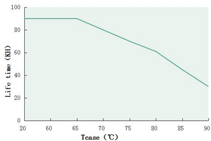
Tcase VS Lifetime (DL-100W-DX-MXG)
