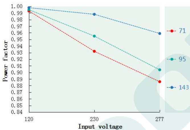
Power factor VS Input voltage(DL-100W-V143DX-MXG)
