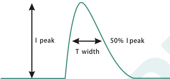
Inrush current(DL-100W-DX-MXG)
