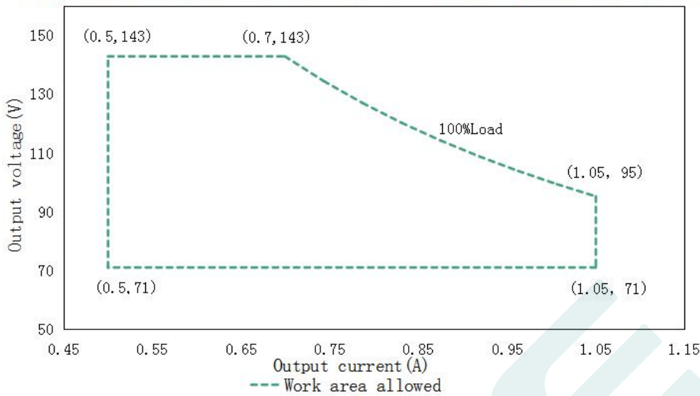
Output voltage VS output current of DL-100W-V143DX-MXG(input: 120-277Vac)
