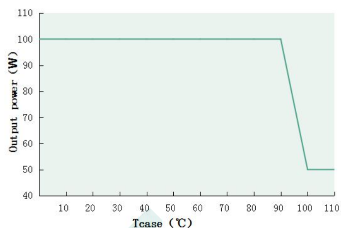
Output power VS Tcase (DL-100W-DX-MXG)
